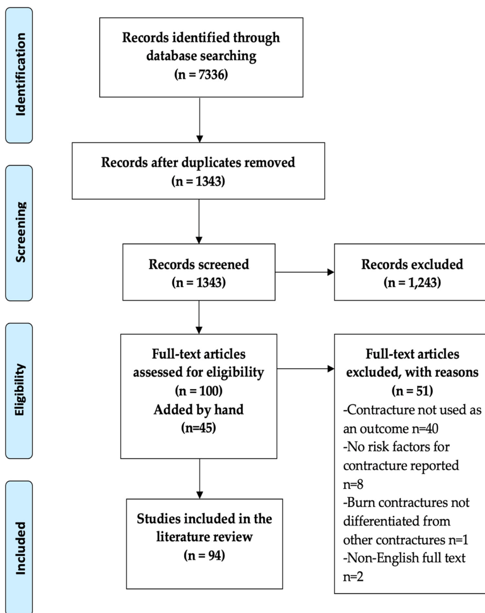
Fig. 1 – PRISMA Chart.
